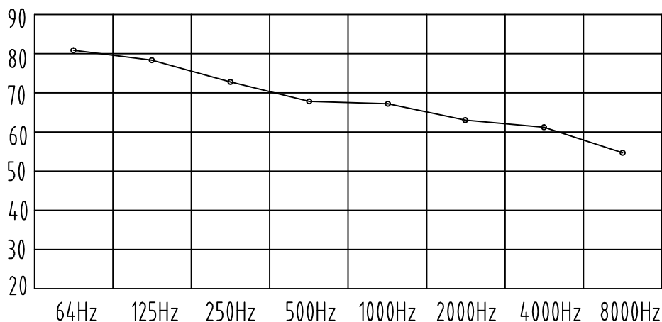
Noise rate analysing chart ( A Class: 72.8dB) dB
